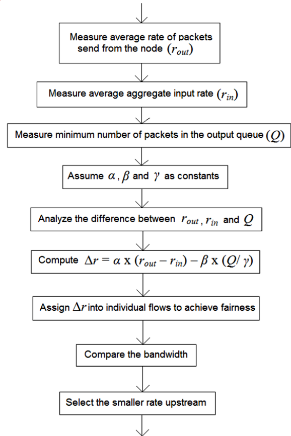
Figure 3 Flowchart for CCF Algorithm
